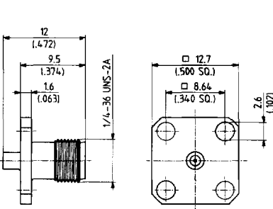
Fig. 1: square flange
