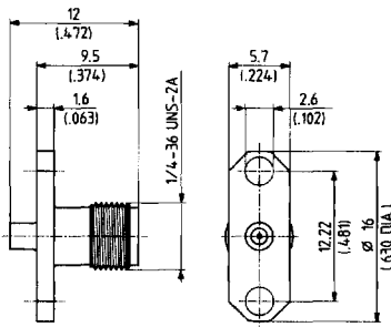
Fig. 2: 2-hole flange
