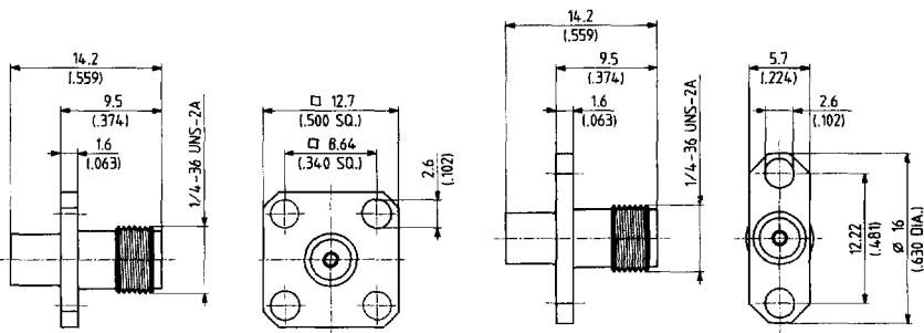
Fig. 1: square flange
