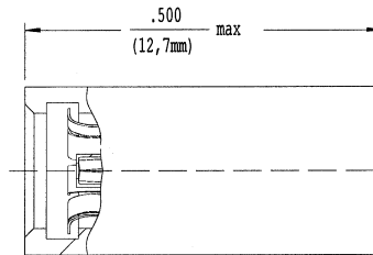
OSSP Blind Mate Jack
