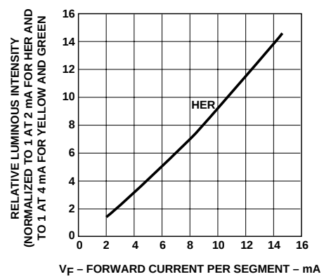
Figure 12. Relative Luminous Intensity vs. DC Forward Current.
