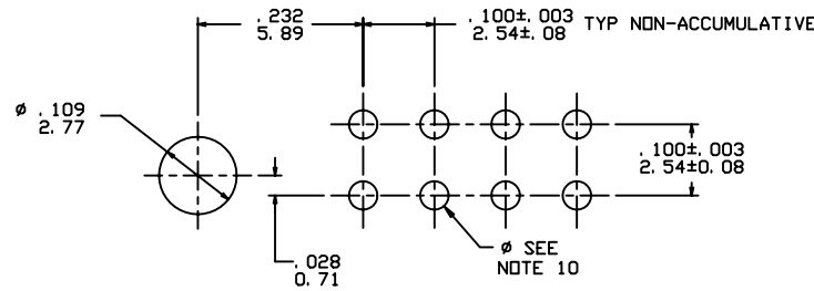
RECOMMENDED HOLE PATTERN SCALE 10:1
