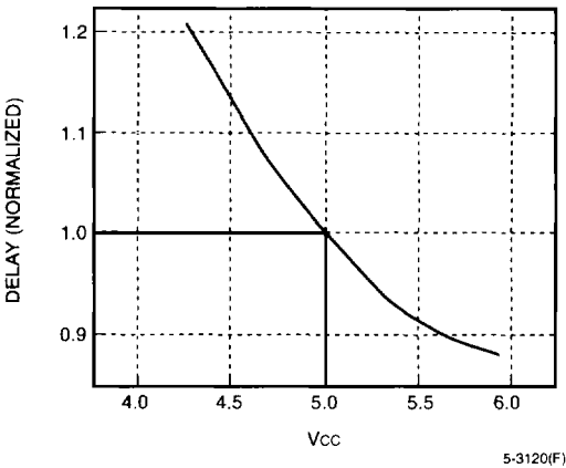
Figure 29. Speed Performance of a CMOS Device
