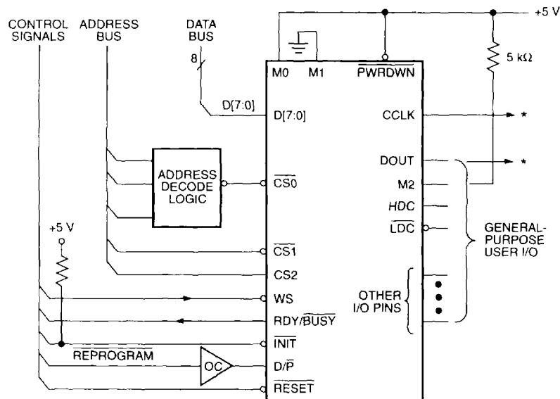
Figure 23. Peripheral Mode
