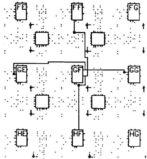
Figure 11. Direct Interconnect
