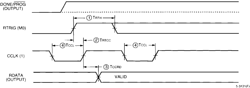
Figure 41. Program Readback Switching Characteristics
