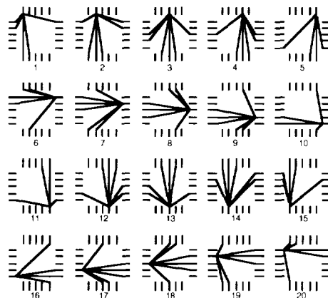
Figure 10. Switch Matrix Interconnection Options
