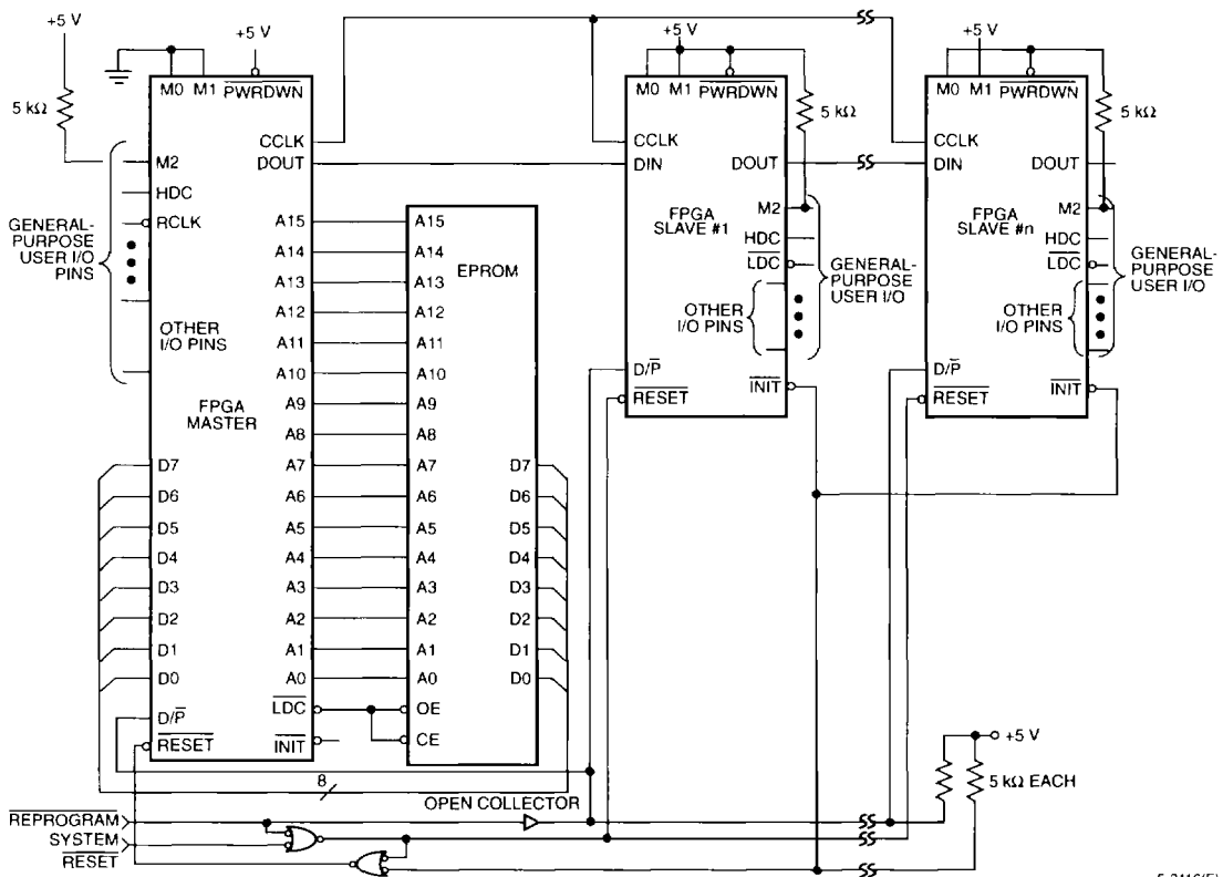
Figure 25. Master Mode with Daisy-Chained Slave Mode Devices
