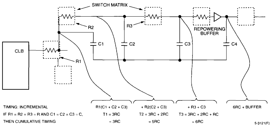
Figure 30. Interconnection Timing Example
