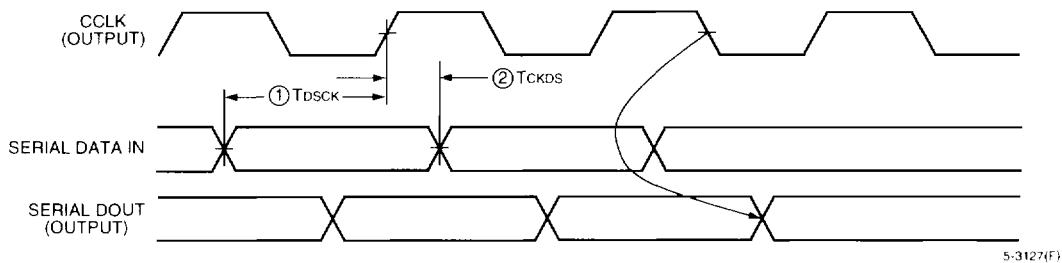
Figure 37. Master Serial Mode Switching Characteristics
