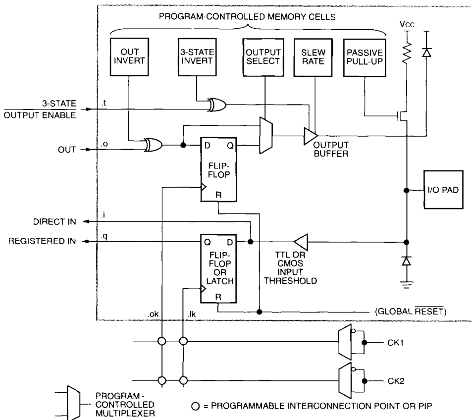
Figure 3. Input/Output Block
