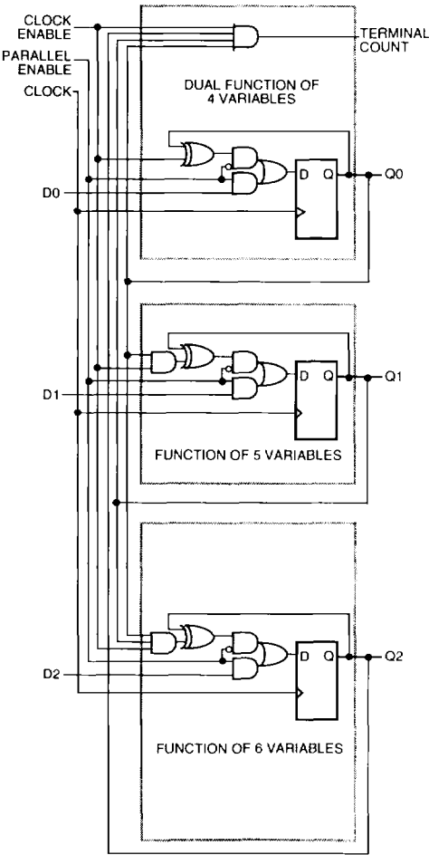
Figure 6. C8BCP Macro
