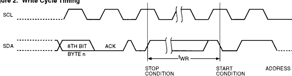
Figure 2. Write Cycle Timing
