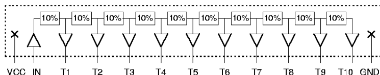
Functional diagram for dash numbers \geq 50
