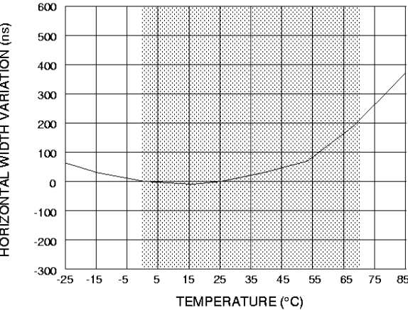
Fig. 12 Horizontal Width Variation vs Temperature
