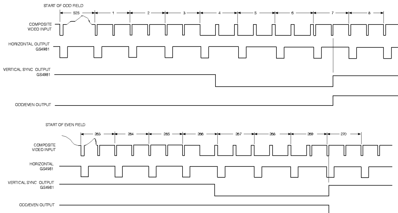
Fig. 28 Timing Diagram
