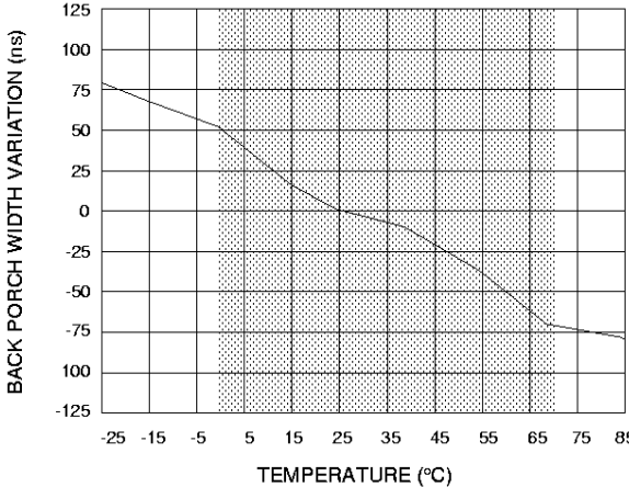
Fig. 10 Back Porch Width Variation vs Temperature
