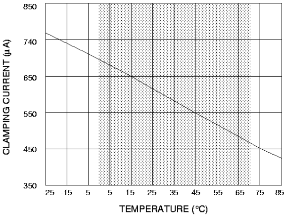
Fig. 8 Clamping Current vs Temperature
