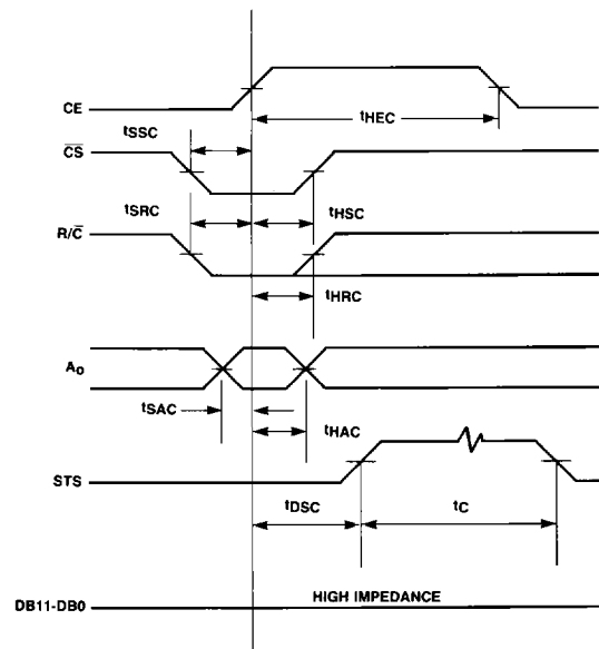
Figure 1. Convert Mode Timing Diagram
