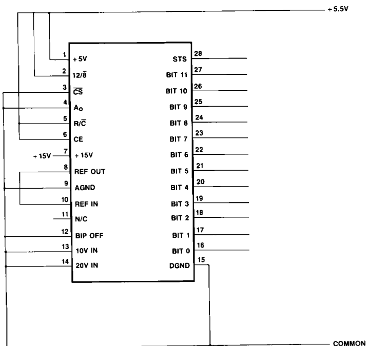
Figure 12. Burn-In Schematic
