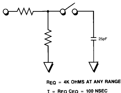
Figure 6. Equivalent HS 574A Input Circuit
