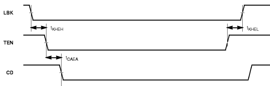
Figure 23. Mode 2 Loopback Timing
