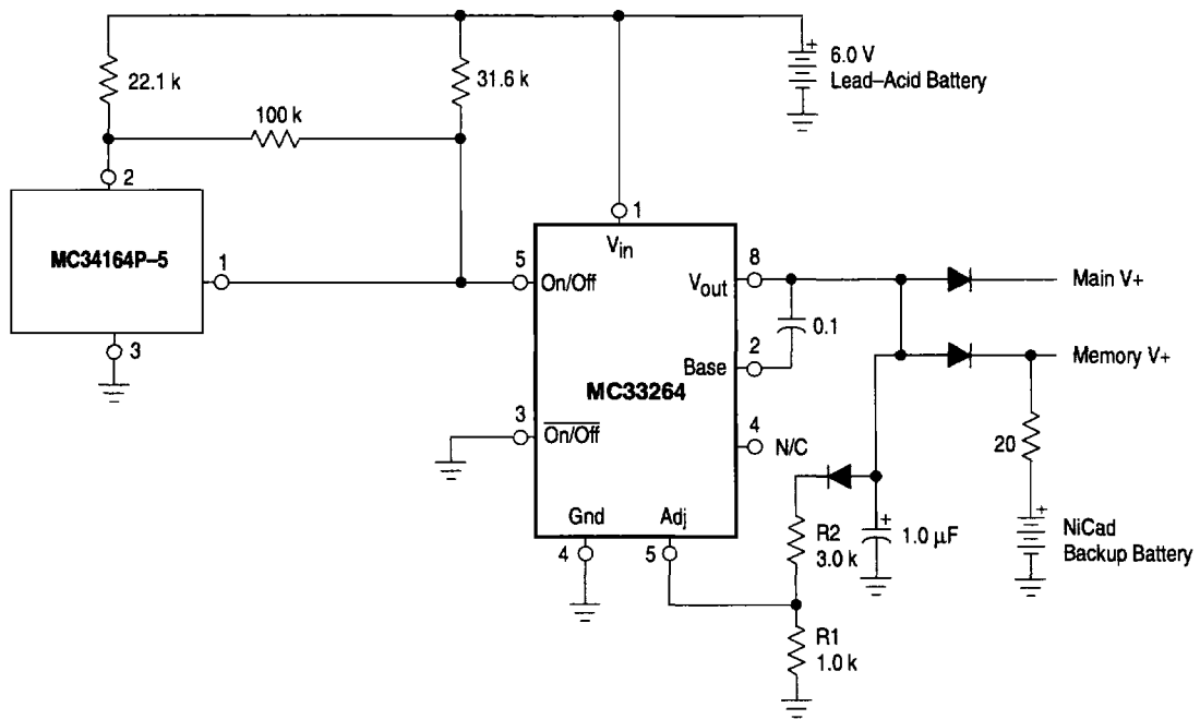
Figure 11. Low Battery Disconnect
