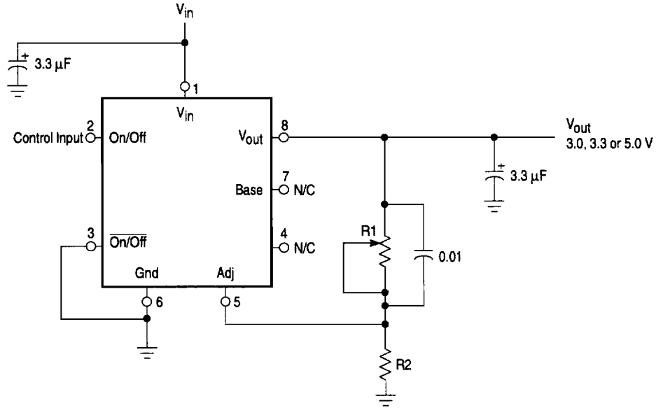
Figure 7. Regulator Output Voltage Trim
