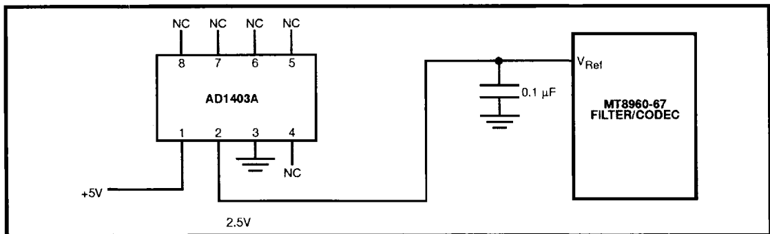
Figure 5 - Typical Voltage Reference Circuit
