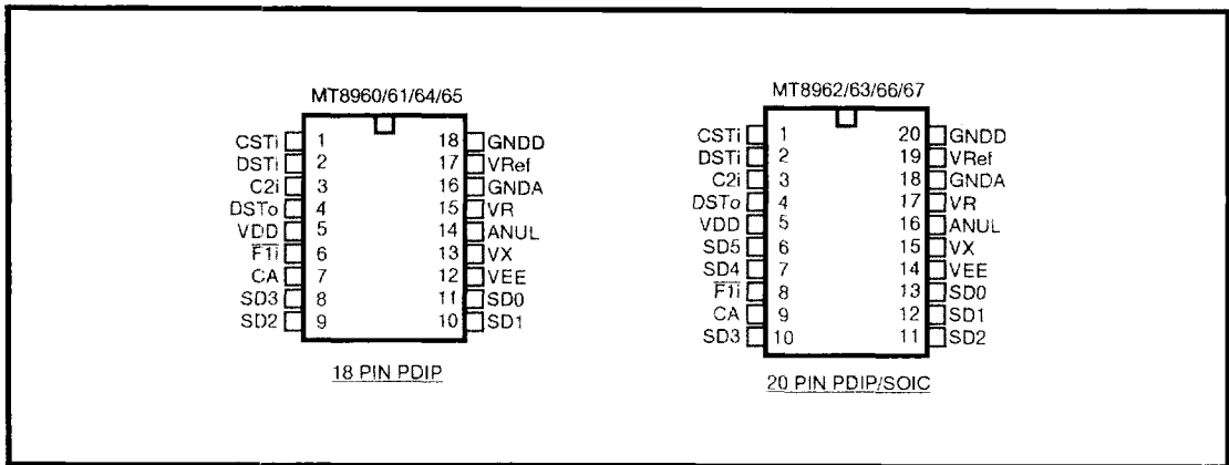
Figure 2 - Pin Connections
