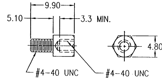
FEMALE SCREWLOCK (SEE ORDERING DATA LEGEND)
