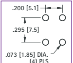
PC MOUNT
