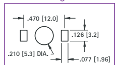
Mounting Detail
