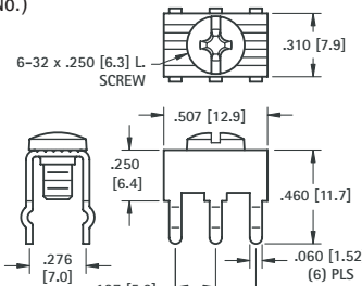
Mounting Detail
