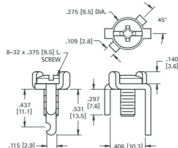
Mounting Detail
