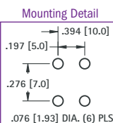
Mounting Detail
