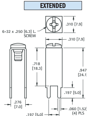
PC MOUNT
