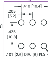
Mounting Detail
