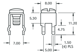
M3 VERTICAL
