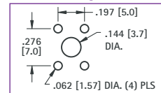
Mounting Detail
