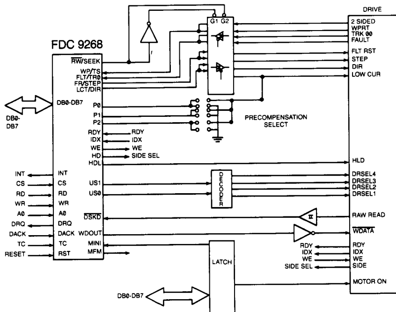
FIGURE 2: TYPICAL APPLICATION
