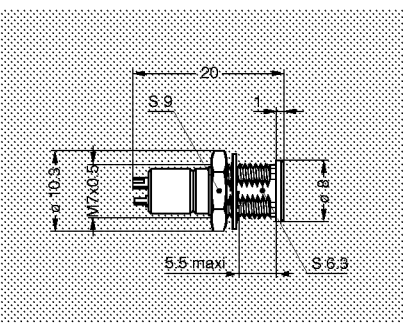
ERM Fixed socket, nut fixing, with microswitch
