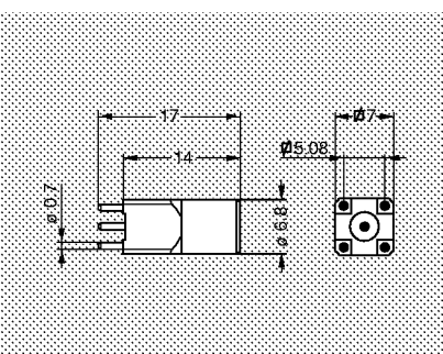
EPC Straight socket for printed circuit with clearance under the body
