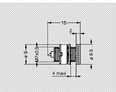
ECP Fixed socket with two nuts
