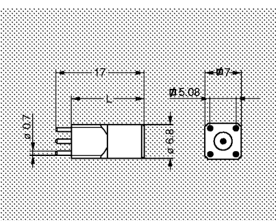
EPA-EPB Straight socket for printed circuit
