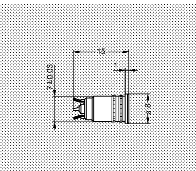
ERT Straight socket without thread, force or adhesive fit
