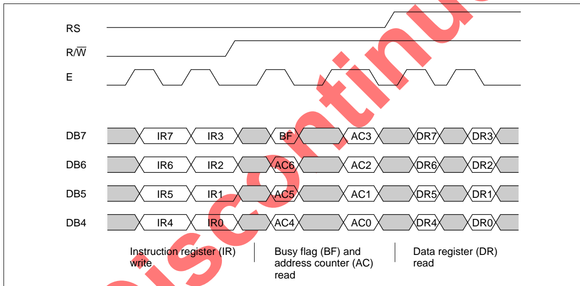
Figure 9 4-Bit Transfer Example
