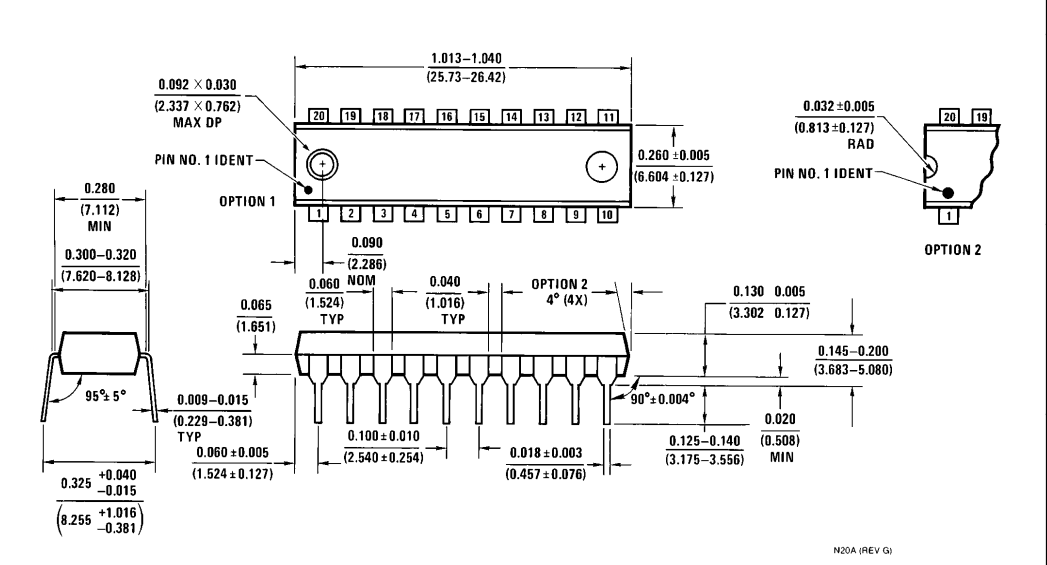
20-Lead (0.300" Wide) Molded Dual-In-Line Package (P) NS Package Number N20A
