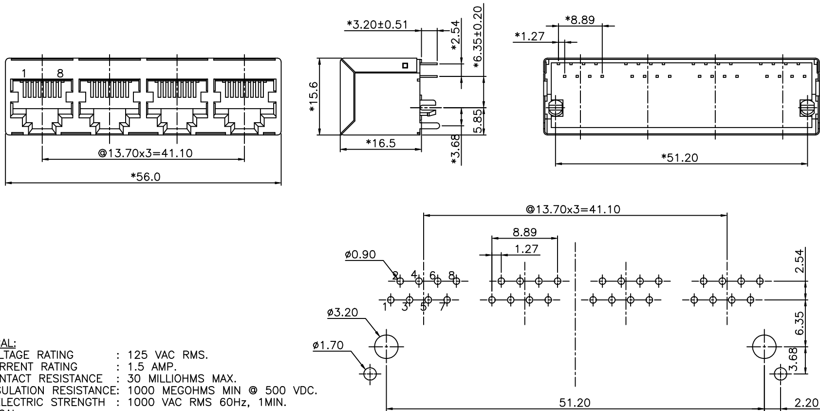
PC Board Layout Component Side Shown
