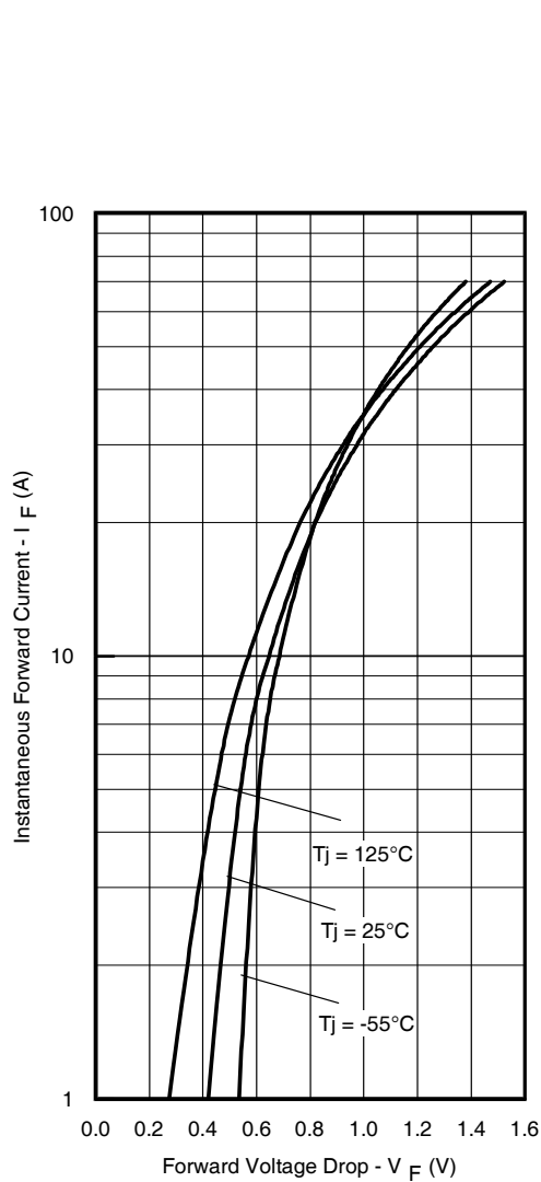
Fig. 1 - Max. Forward Voltage Drop Characteristics
