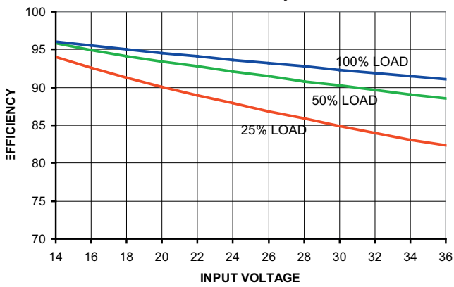
7812SR Efficiency
