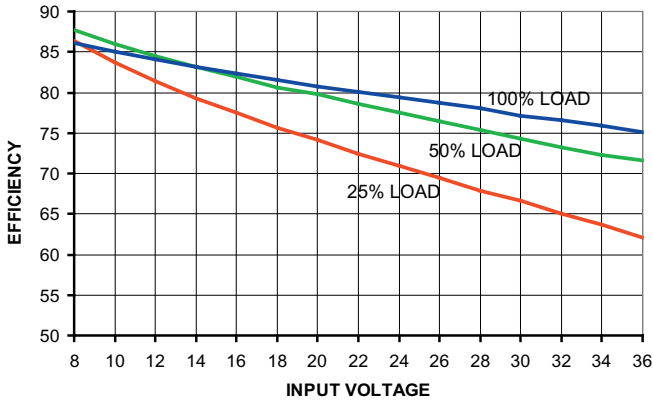
7803SR Efficiency
