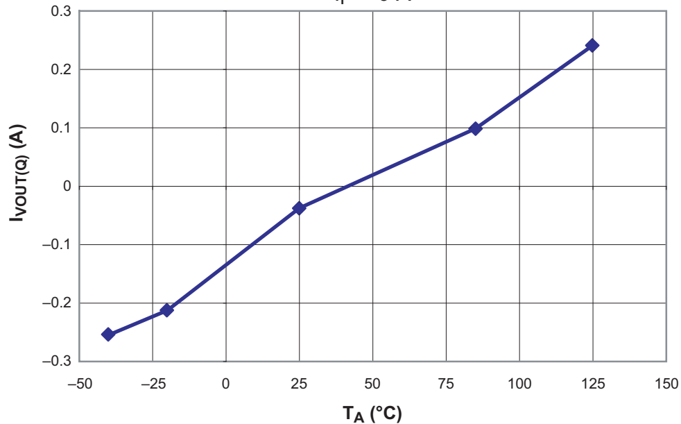
Zero Current Output Current versus Ambient Temperature
