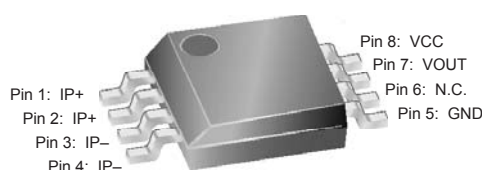
Package LC
