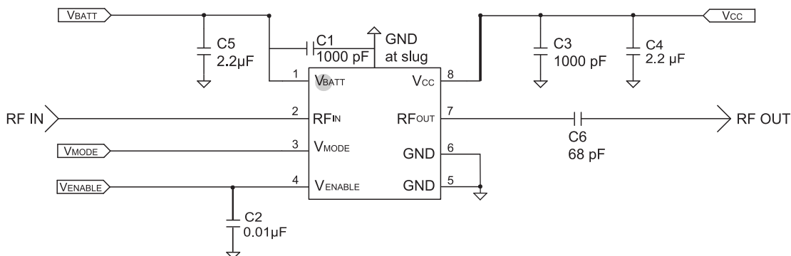
Figure 3: Application Circuit
