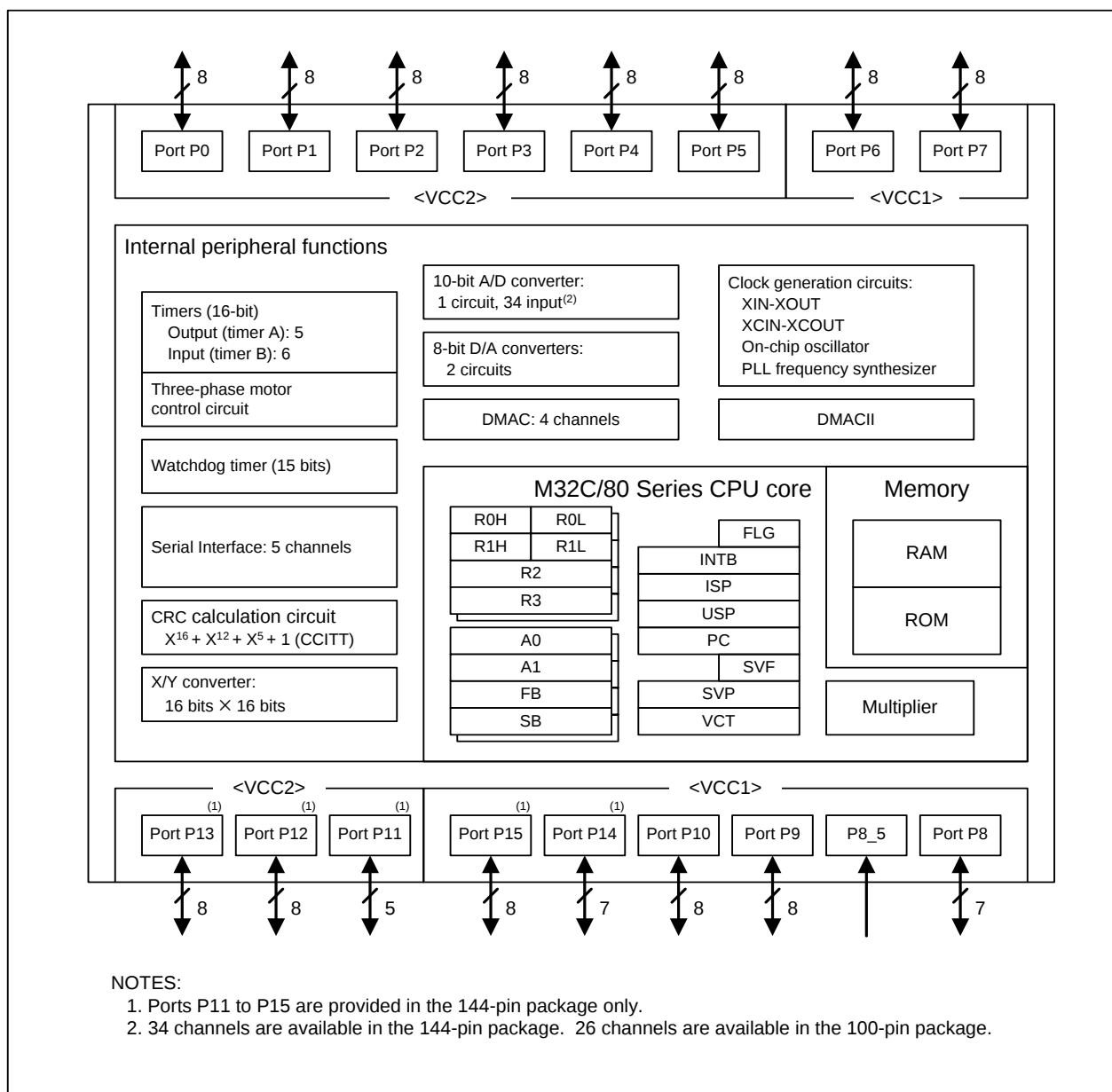
Figure 1.2 Block Diagram
