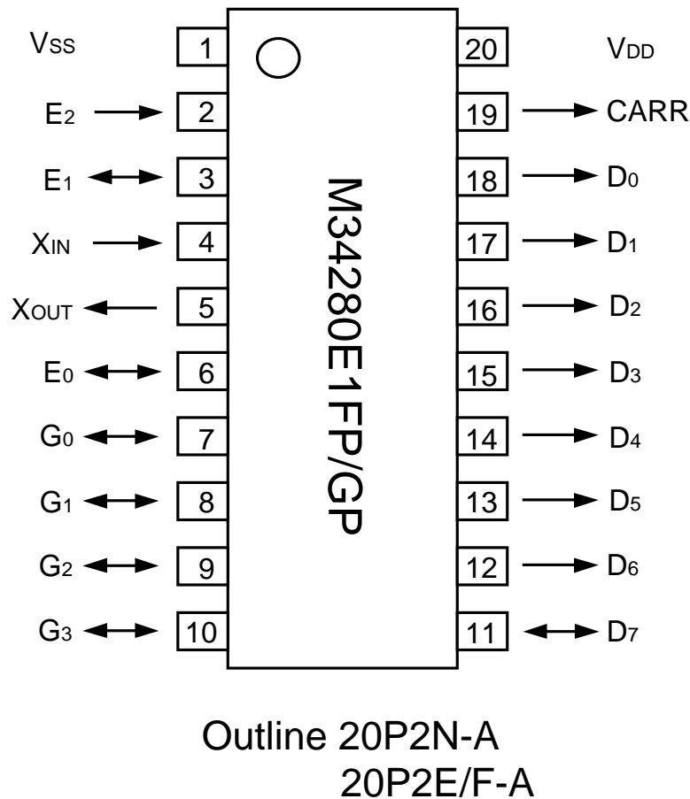
Fig. 26 Pin configuration of built-in PROM version
