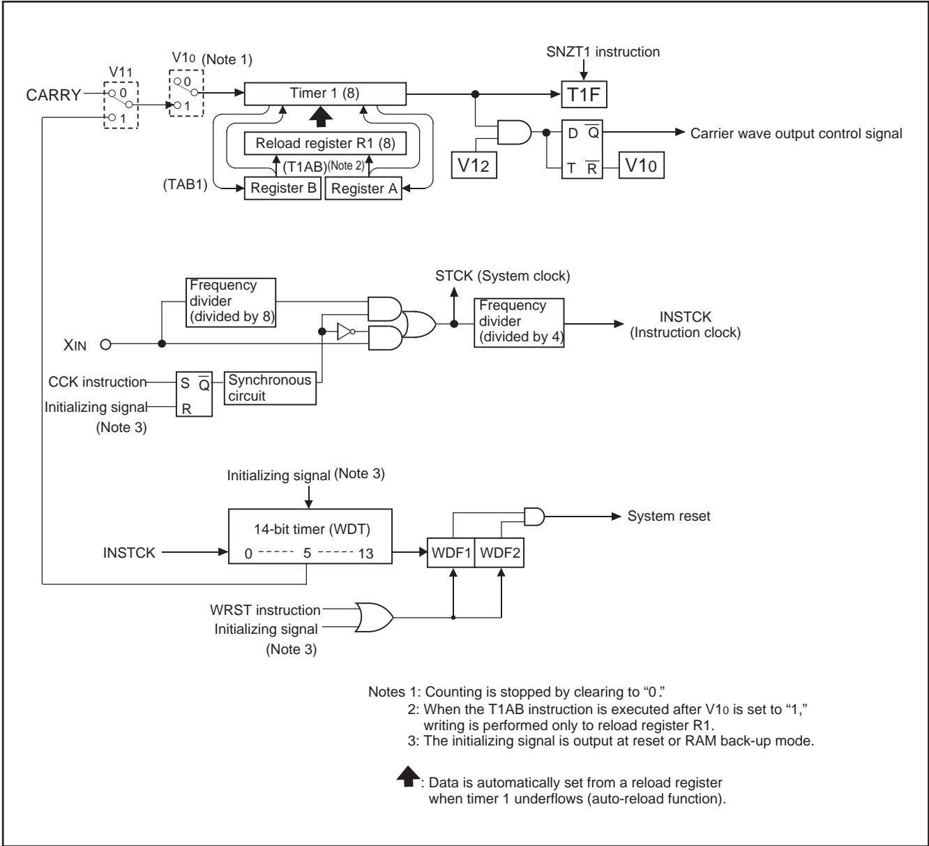
Fig. 13 Timers structure
