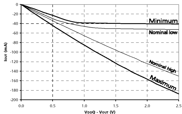
Figure 10: Pull-Up Characteristics
