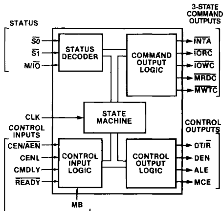
Figure 1. 82288 Block Diagram
