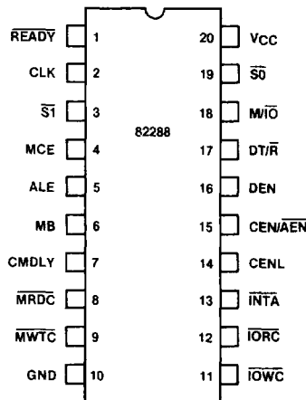
Figure 2. 82288 Pin Configuration
