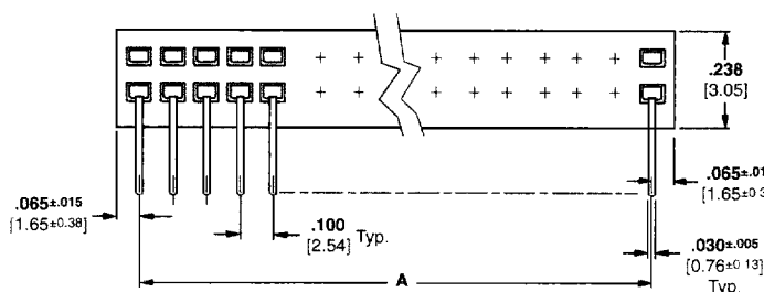
Housing Configuration 1
