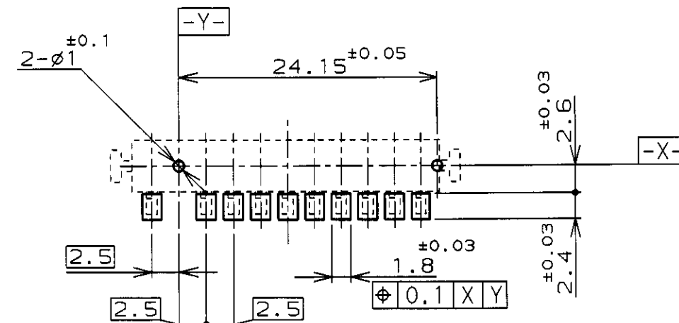
基板取付推奨寸法 RECOMMENDED P.C. BOARD LAYOUT P.C. BOARD THK 0.8~1.2 (VIEW FROM CONNECTOR MOUNTING SIDE)
