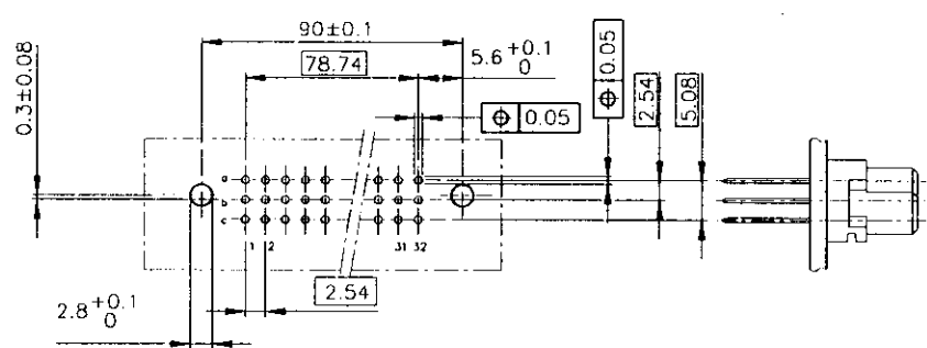
P.C. MOUNTING HOLE PATTERN
