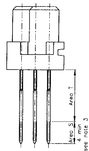
Detail X scale 5:1
