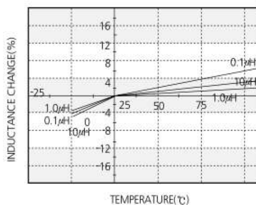
(4) Temperature Characteristics
