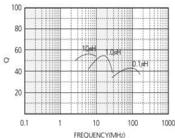
(2) Q Characteristics
