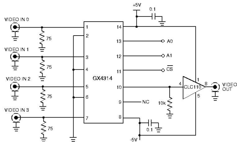
Fig. 7 Test Circuit
