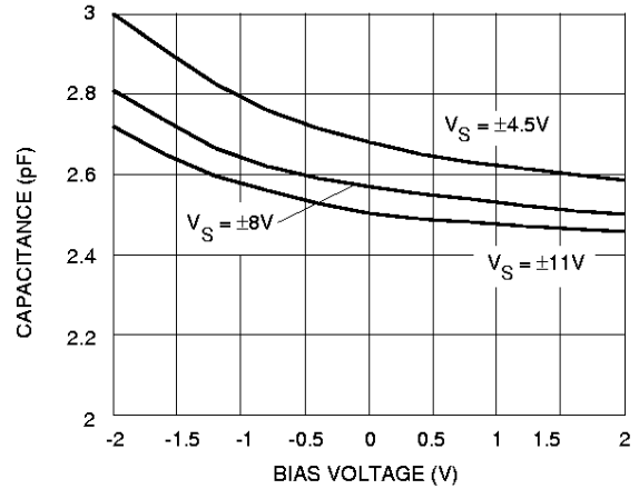
Fig. 4 Output Capacitance
