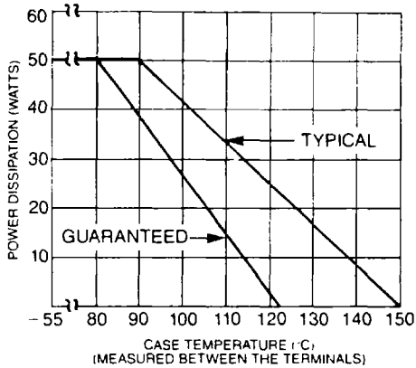
POWER DERATING
