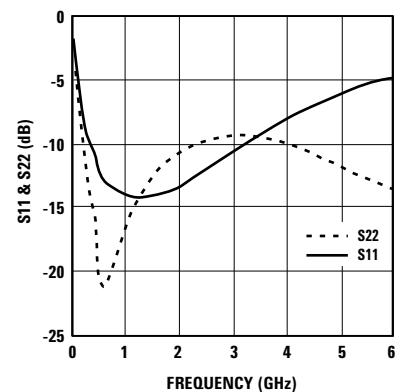
Figure 7. S11 and S22 (50Ω) vs. Frequency.
