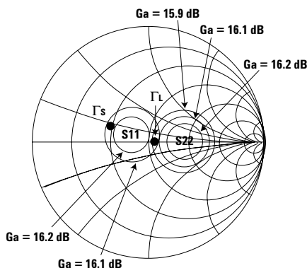
Figure 18. Input and output gain circles.
