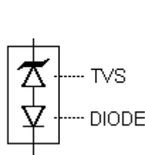
FIGURE 2 TVS with internal Low Capacitance Diode
