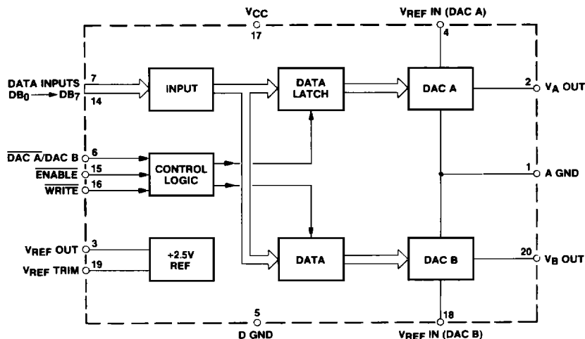
Fig 1 System diagram
