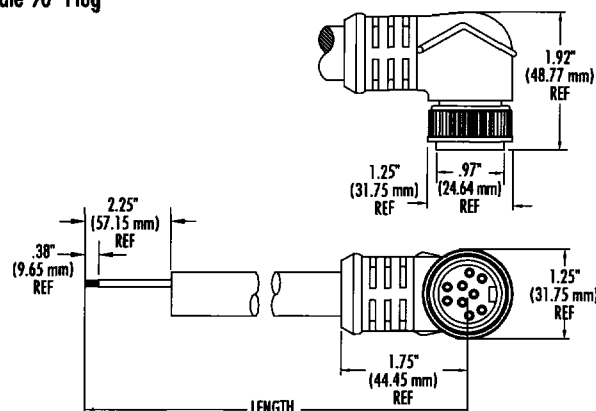
Male 90° Plug
