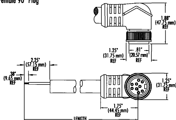
Female 90° Plug
