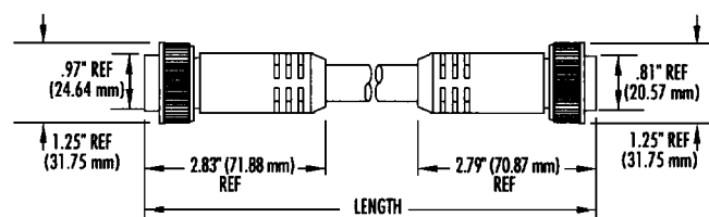
Male/Female Cable Assembly
