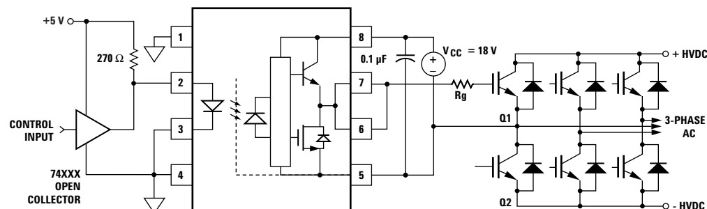
Figure 25. Recommended LED Drive and Application Circuit
