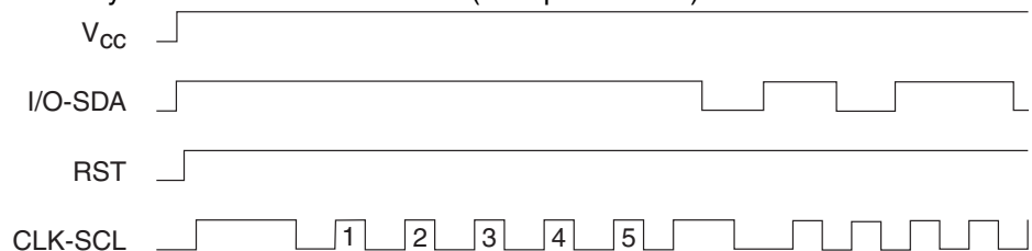
Figure 3. Synchronous 2-wire Protocol (Gemplus Patent)
