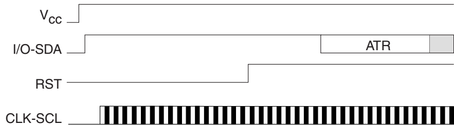
Figure 2. Asynchronous T = 0 Protocol (Gemplus Patent)
