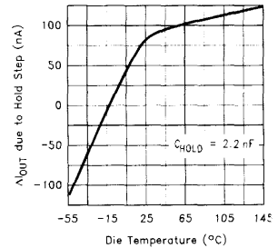
Hold Step (I OUT ) vs Temperature
