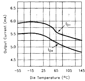
Output Current Swing vs Temperature (Sample & Hold)
