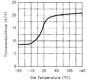
Transconductance vs Temperature (Sample & Hold)
