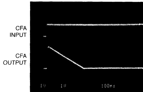
Figure 5. Autozero Mechanism Restores Amplifier Output to Ground after +1\text{V} Step at Input
