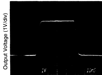
Large-Signal Step Response
