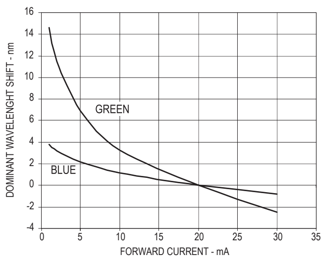
Figure 9. Relative dominant wavelength vs Forward Current
