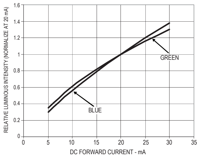
Figure 7. Relative Intensity vs Forward Current
