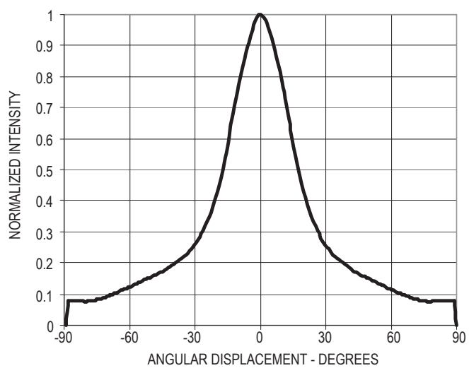
Figure 11. Radiation Pattern – Minor Axis
