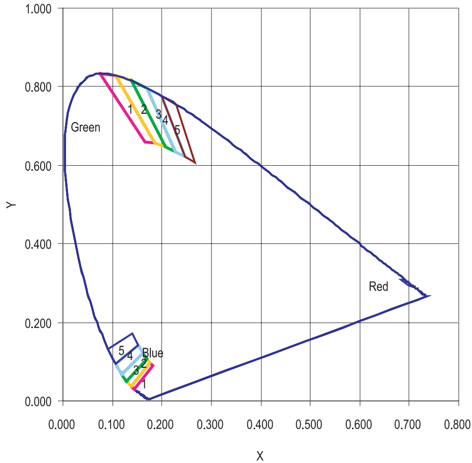
Avago Color Bin on CIE 1931 Chromaticity Diagram
