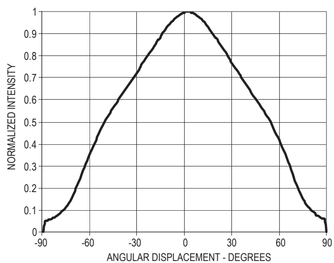
Figure 10. Radiation Pattern – Major Axis
