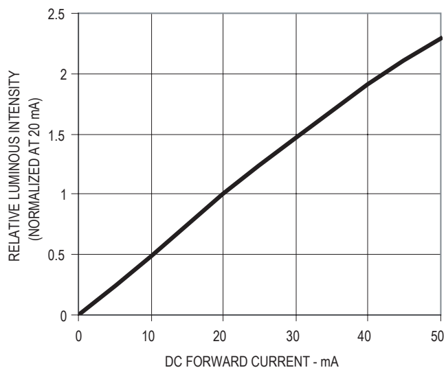
Figure 3. Relative Intensity vs Forward Current
