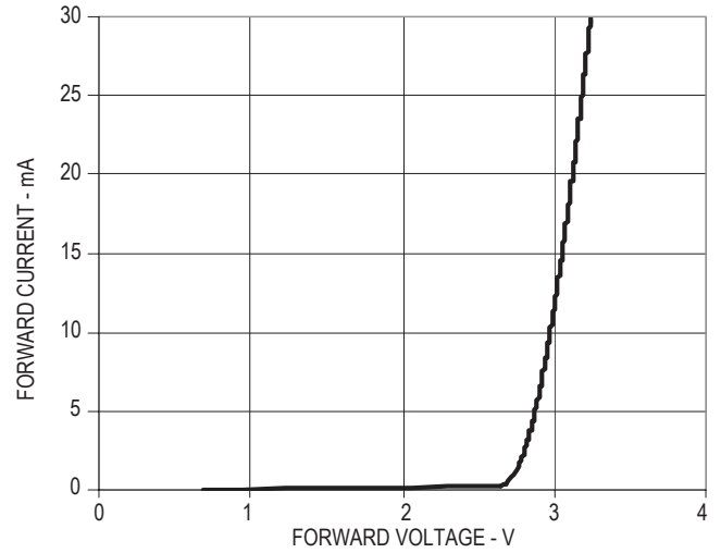
Figure 6. Forward Current vs Forward Voltage
