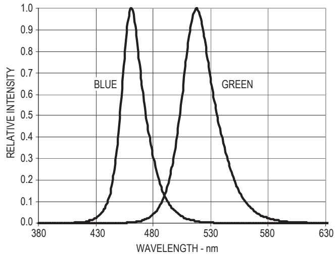
Figure 5. Relative Intensity vs Wavelength
