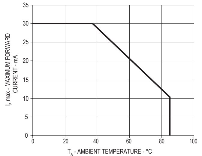
Figure 8. Maximum Forward Current vs Ambient Temperature
