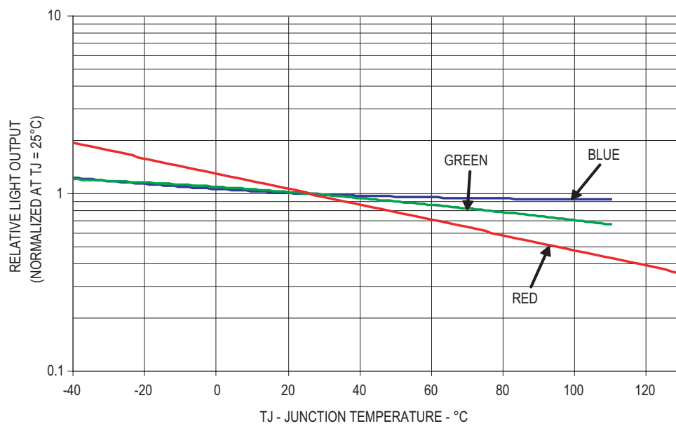
Relative Light Output vs Junction Temperature
