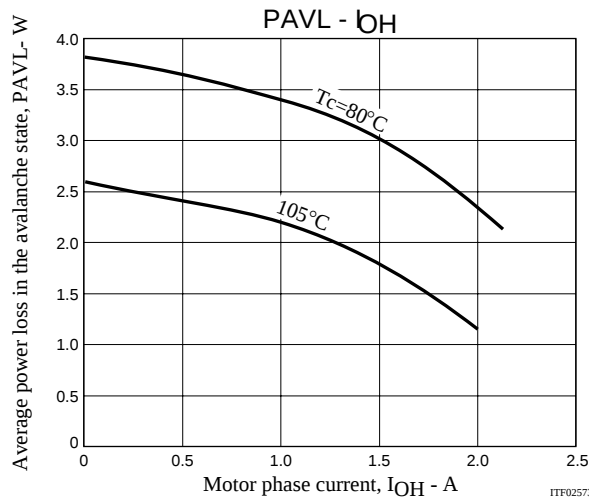
Figure 3 Allowable Loss Range, PAVL-I_{OH} During STK672-630A-E Avalanche Operations
