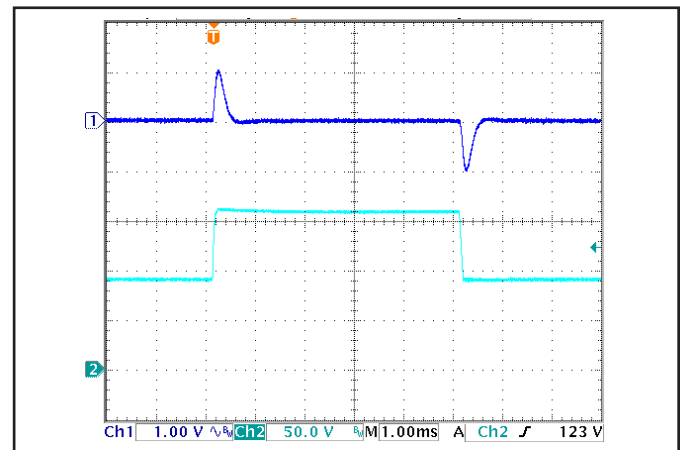
Figure 6: Output voltage response to step-change in input voltage (1000 V/ms). Load cap: 100 μF, electrolytic output capacitance. Ch 1: V out (1 V/div), Ch 2: V in (50 V/div).
