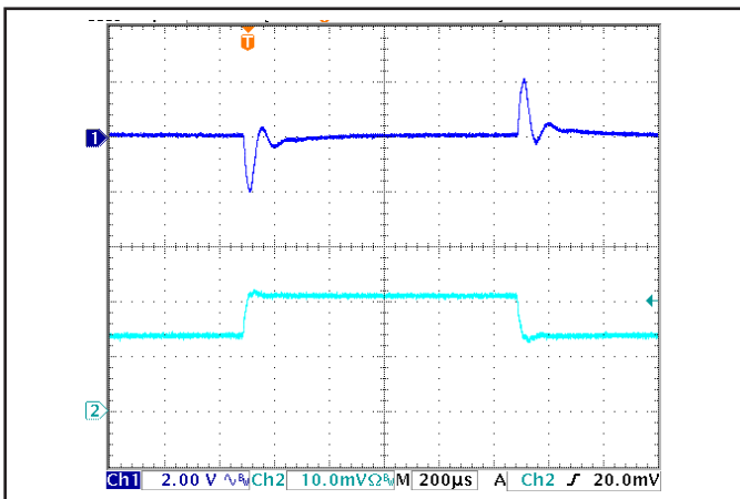
Figure 5: Output voltage response to step-change in load current (50%-75%-50% of I out (max); dI/dt = 0.05 A/μs). Load cap: 1 μF ceramic capacitor. Ch 1: V out (2 V/div), Ch 2: I out (2 A/div).
