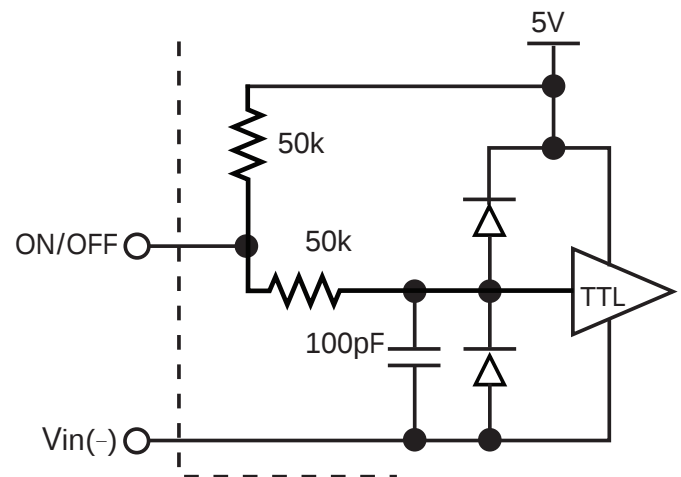
Figure B: Internal ON/OFF pin circuitry
