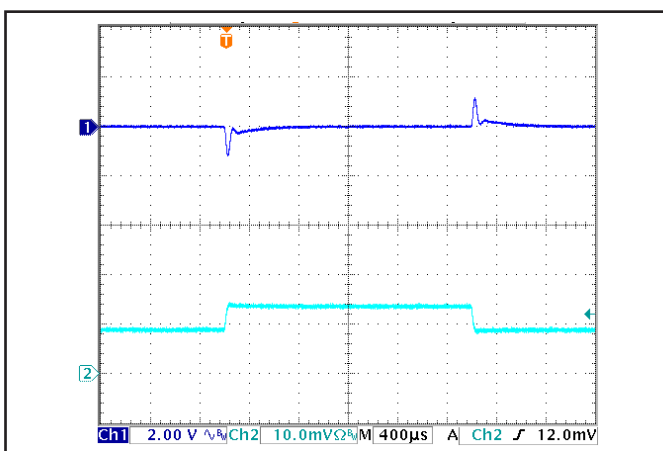
Figure 5: Output voltage response to step-change in load current (50%-75%-50% of Iout(max); dI/dt = 0.1 A/μs). Load cap: 1 μF ceramic capacitor. Ch 1: Vout (2 V/div), Ch 2: Iout (5 A/div).
