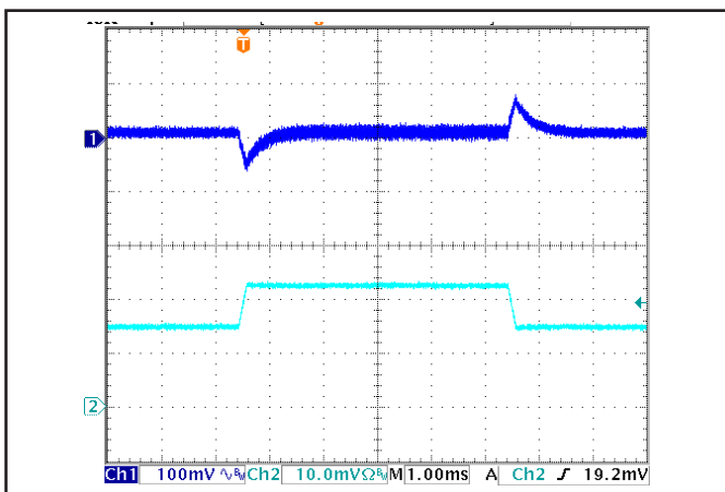
Figure 5: Output voltage response to step-change in load current (50%-75%-50% of Iout(max); dI/dt = 0.1 A/μs). Load cap: 1 μF ceramic and 15 μF tantalum capacitors. Ch 1: Vout (100 mV/div), Ch 2: Iout (20 A/div).
