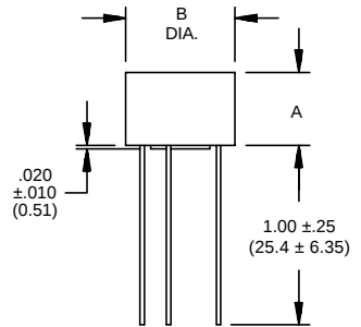
TERMINAL ARRANGEMENT A
