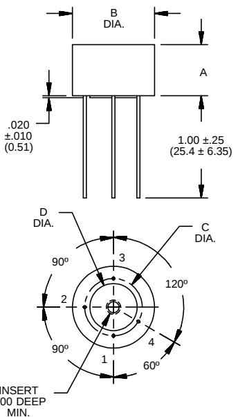
TERMINAL ARRANGEMENT B
