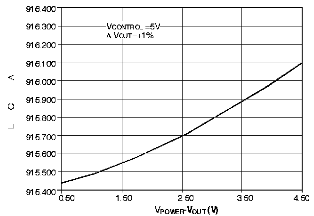
Minimum Load Current vs V_{\text{POWER}} - V_{\text{OUT}}
