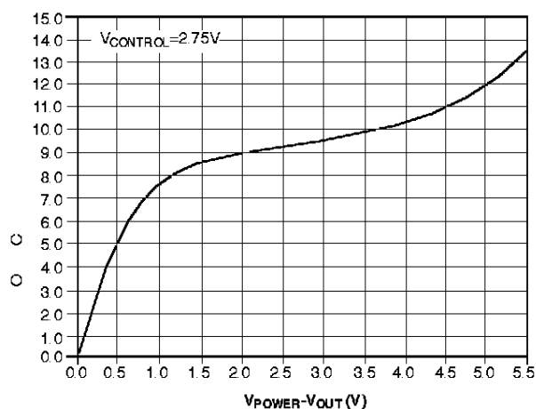
Short Circuit Current vs V_{\text{POWER}} - V_{\text{OUT}}
