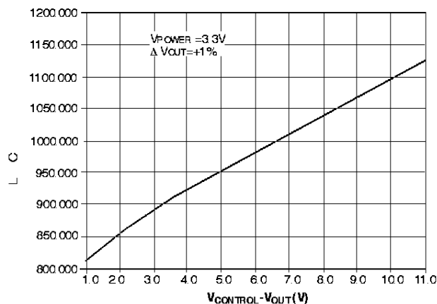
Minimum Load Current vs V_{\text{CONTROL}} - V_{\text{OUT}}
