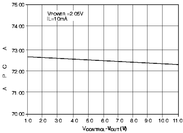
Adjust Pin Current vs V_{\text{CONTROL}} - V_{\text{OUT}}
