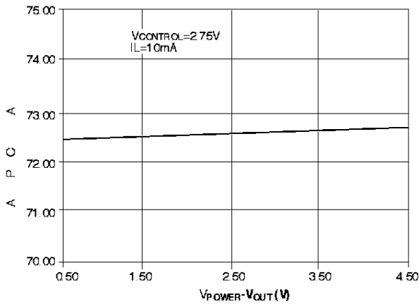
Adjust Pin Current vs V_{\text{POWER}} - V_{\text{OUT}}
