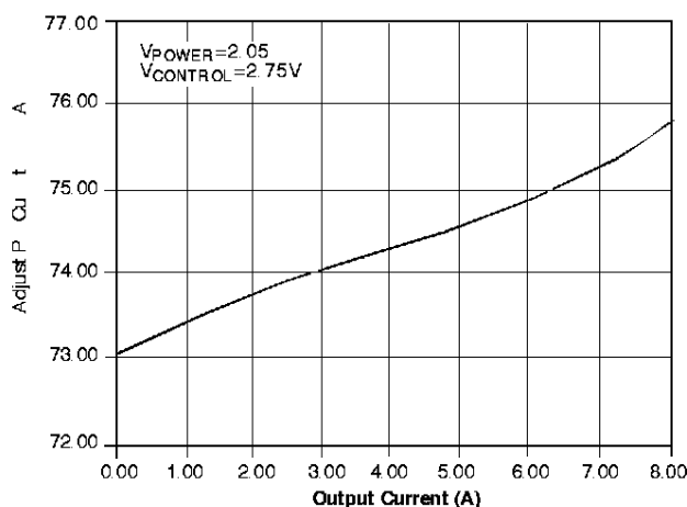
Adjust Pin Current vs. Output Current
