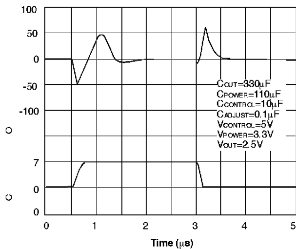
Transient Response
