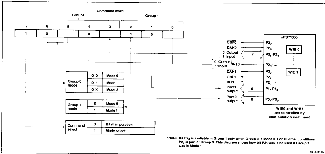
Figure 11. Mode 1 Output
