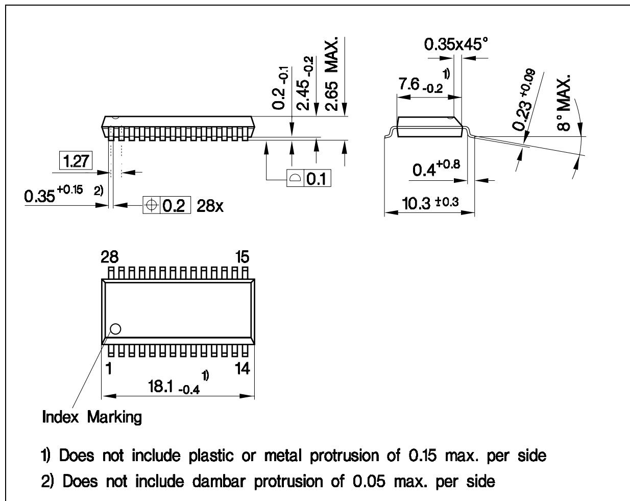
Figure 8 P-DSO-28-1 Package
