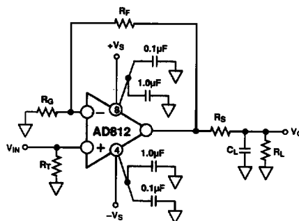
Figure 38. Circuit for Driving a Capacitive Load
