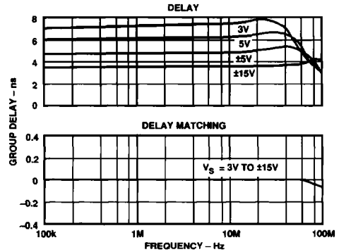
Figure 49. Group Delay and Group Delay Matching vs. Frequency, Gain = +2, R_L = 150 \Omega
