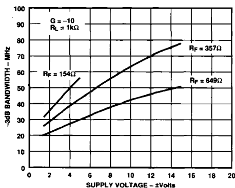
Figure 36. -3 dB Bandwidth vs. Supply Voltage, Gain = -10, R_L = 1 k\Omega
