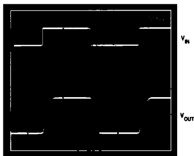
Figure 41. Pulse Response of Circuit of Figure 38 with C_L = 510\text{ pF} , R_L = 1\text{ k}\Omega , R_F = R_G = 715\ \Omega , R_S = 15\ \Omega
