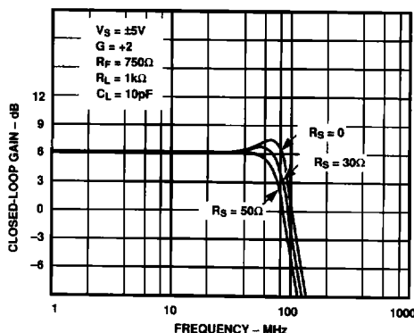
Figure 39. Response to a Small Load Capacitor at \pm 5 V
