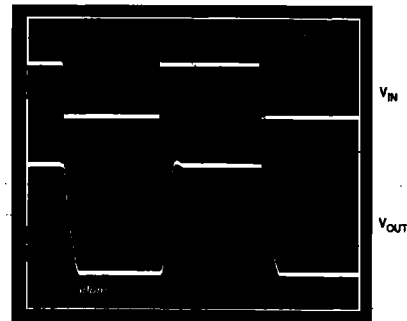
Figure 52. Pulse Response of the Circuit of Figure 50 with V_s = 5 V
