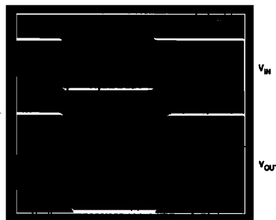
Figure 42. 6 dB Overload Recovery; G = 10 , R_L = 500\ \Omega , V_s = \pm 5\text{ V}
