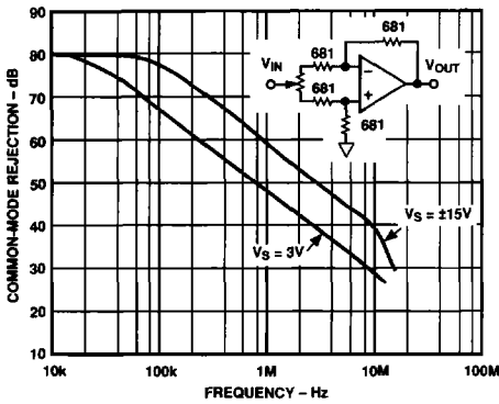
Figure 14. Common-Mode Rejection vs. Frequency
