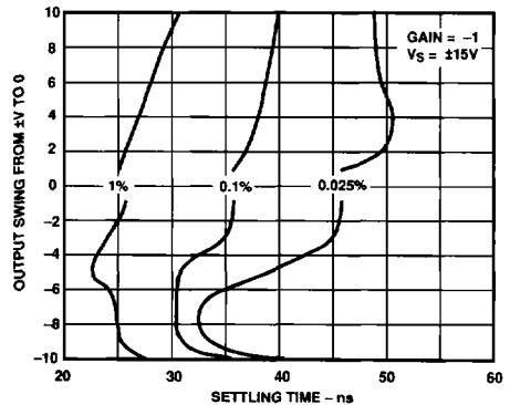
Figure 18. Output Swing and Error vs. Settling Time
