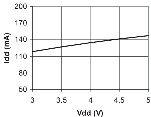
Figure 8. I_{dd} Over V_{dd} (same V_g )
