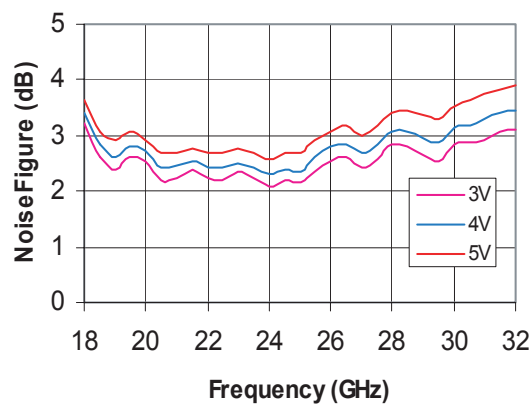
Figure 10. Noise Figure Over V_{dd}
