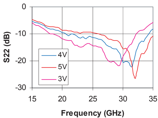
Figure 12. Output Return Loss Over V_{dd}
