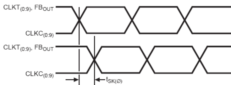
Figure 7. Output Skew
